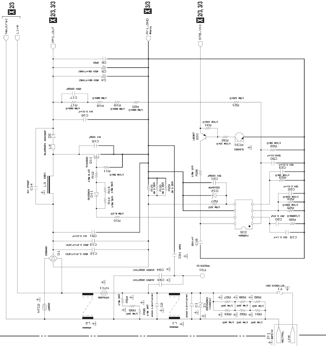
X 1/3 SW POWER SUPPLY (DWR1549)
